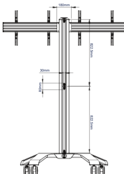
REAR VIEW
