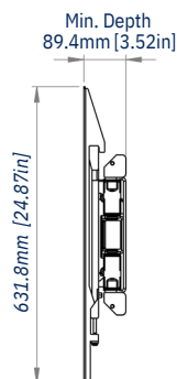
SIDE VIEW FLAT TO WALL
