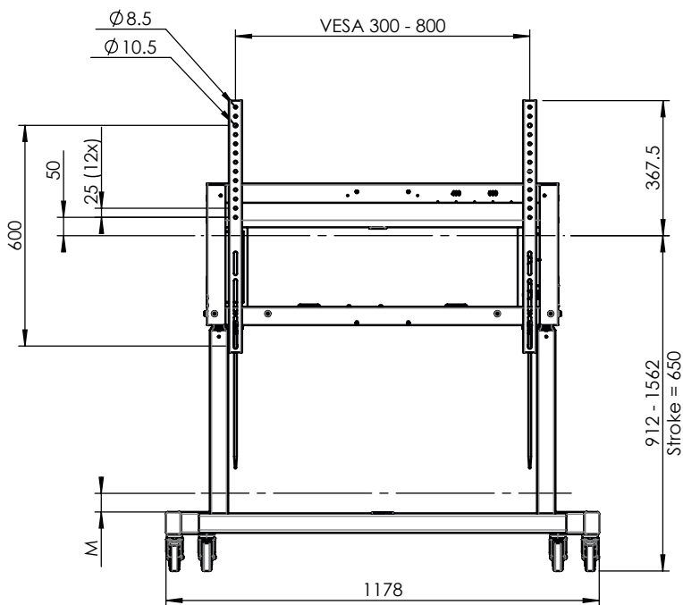
M = minimal free space of 51mm
